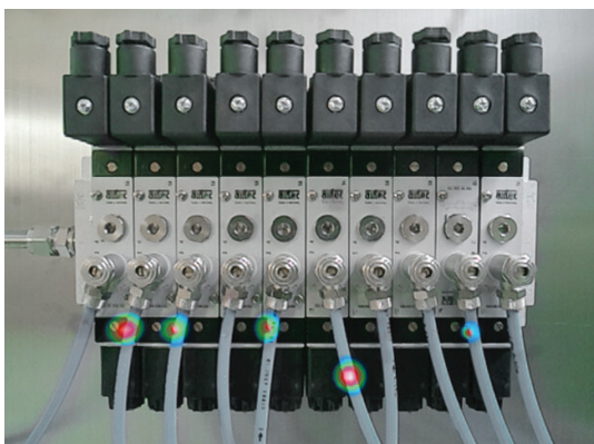
LeakCam 600 with 64 microphones (Power Beam Forming)
